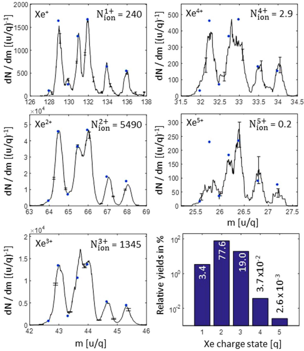
Fig. 2. TOF spectra of Xe at 93 eV. Measured mass spectra of the xenon charge states \text{Xe}^{q+} ( q = 1, \dots, 5 ) generated by photoionization of xenon atoms in the focus of the 93-eV XUV beam. The signal corresponds to the number of ions per unit mass-to-charge ratio m detected in a field of view of 395 \mu\text{m} in diameter. The number N_{\text{ion}}^{q+} in the right upper corner of each graph corresponds to the number of ions \text{Xe}^{q+} generated per shot in the field of view of the IM, taking into account the 50% detection efficiency. The blue markers indicate the expected positions and frequencies of the seven stable xenon isotopes. The relative photoionization yields of all the measured charge states are shown in the lower right panel.
