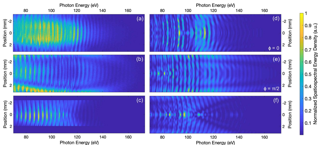
Fig. 2. Single-shot measurement of the spatiotemporal energy density distribution of the XUV beam generated from the 1.5 mm neon gas jet, exhibiting (a) on-axis and (b) off-axis emission. In the experiment, the spatial energy-density distribution varies randomly from shot to shot (see additional shots in Supplement 1). (c) Single-shot measurement of the spatiotemporal energy density distribution of the XUV beam generated from the 5 cm gas cell. Significant energy is present off-axis in comparison to Fig. 1, (a)–(b), showing also a higher cutoff energy. Additionally, spectral modulations are visible throughout the whole measured region, not allowing the isolation of single pulses. The lack of signal at radii above 2 mm is due to changes in the detector’s clear aperture, unrelated to these specific measurements. Calculated spatially resolved spectra for a 1.5 mm length gas jet for a CEP value of (d) \phi_{\text{CEP}} = 0 and (e) \phi_{\text{CEP}} = \pi/2 . Only the changes obtained when varying the CEP can accurately reproduce the differences between (a) and (b). (f) Calculated spatially resolved spectra for the 5 cm cell, again reproducing the features of the spectrum shown in (c).
