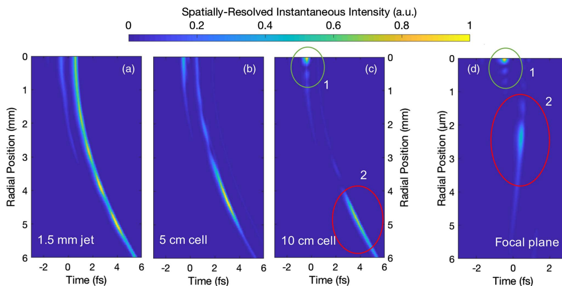
Fig. 4. Normalized spatially resolved instantaneous intensity of harmonics at the cutoff-energy region (115 eV, 11 eV bandwidth), arising from the (a) 1.5 mm jet, (b) 5 cm cell, and (c) 10 cm cell, at the detector plane located 12 m away from the generation target. For the first two cases, the radiation is distributed over a wide area, and double pulses are obtained on axis. However, with the 10 cm long cell, the on- and off-axis radiation (region 1, green circle and region 2, red circle, respectively) becomes spatiotemporally isolated in the detector plane. (d) After focusing the pulses with a 12.5 mm mirror, the spatial separation of the two sequential pulses is maintained due to their different divergence, caused by dynamic wavefront bend of the driving laser.
