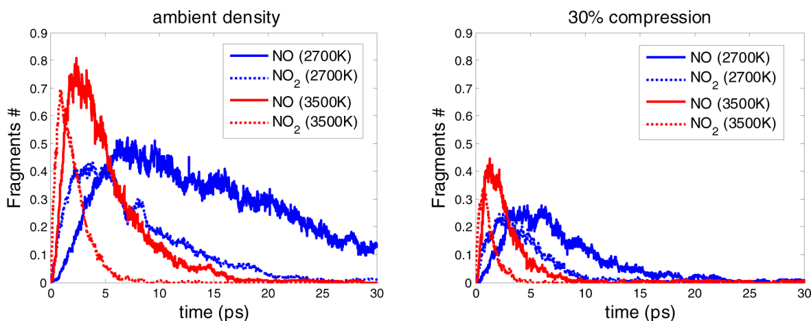
Figure 10. NO and NO 2 formation at ambient density (left) and 30% compression, at 2700 and 3500 K.
