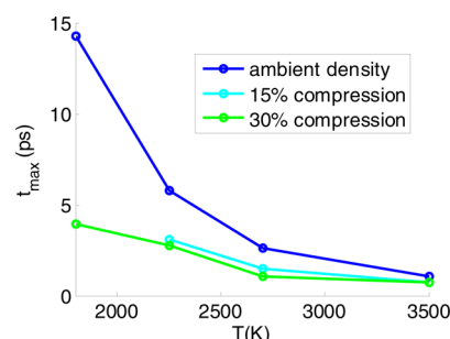
Figure 5. Plot of PE maximum time, t_{\text{max}} (ps) versus temperature (K), for ambient density, and 15 and 30% compressed liquid TNT.
