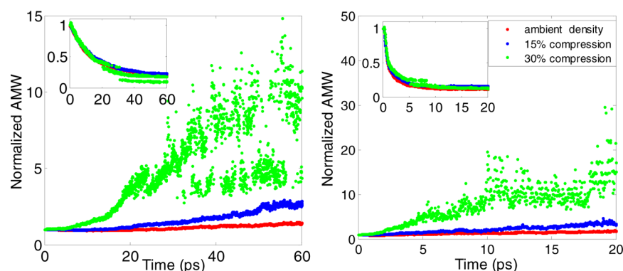
Figure 15. AMW as a function of time at 2250 (left) and 3500 K (right) for ambient density (red) and 15 (blue) and 30% (green) compressions. The results in the main and the internal panels are for C \geq 7 and C \geq 0 , respectively.
